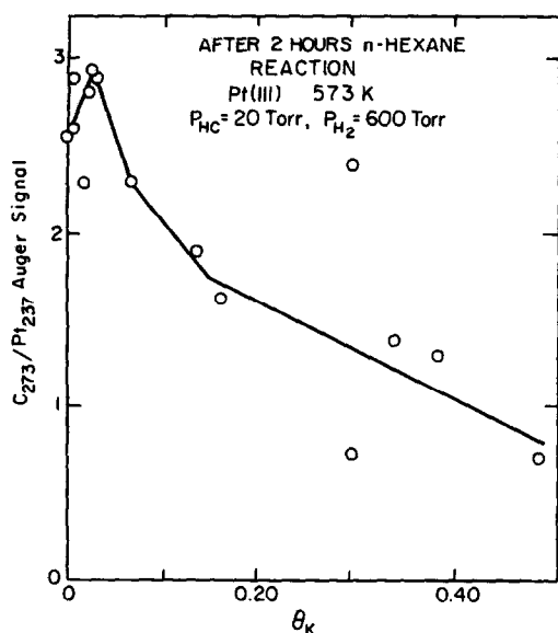
Fig. 6. Carbon to platinum AES signal ratio after n-hexane reaction over Pt(111) surfaces as a function of potassium coverages.
