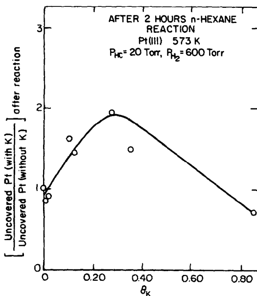
Fig. 8. Fractional concentrations of uncovered platinum surface sites after n-hexane reactions determined by CO titration, as a function of potassium coverage (relative to the same fractional concentration after reaction for the clean platinum case).
