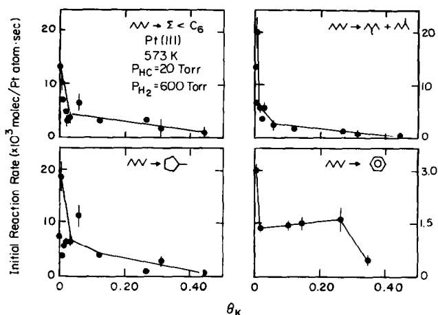
FIG. 2. Initial reaction rates for hydrogenolysis, isomerization, cyclization, and aromatization of n-hexane over Pt(111) surfaces as a function of potassium coverages.
