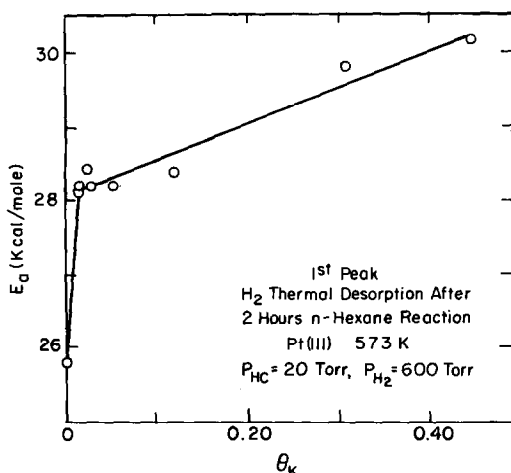
FIG. 10. Activation energy of the hydrogen \beta -elimination from the carbonaceous deposits after n-hexane reactions over Pt(111) surfaces as a function of potassium coverages.
