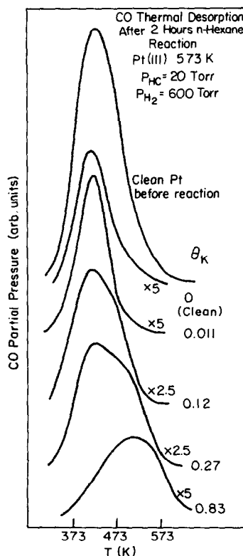
Fig. 7. CO thermal desorption spectra following CO saturation of the Pt(111) surface after 2 h of n-hexane reaction for different potassium coverages. The adsorption temperature was 300–310 K, the heating rate 80 K/s.
