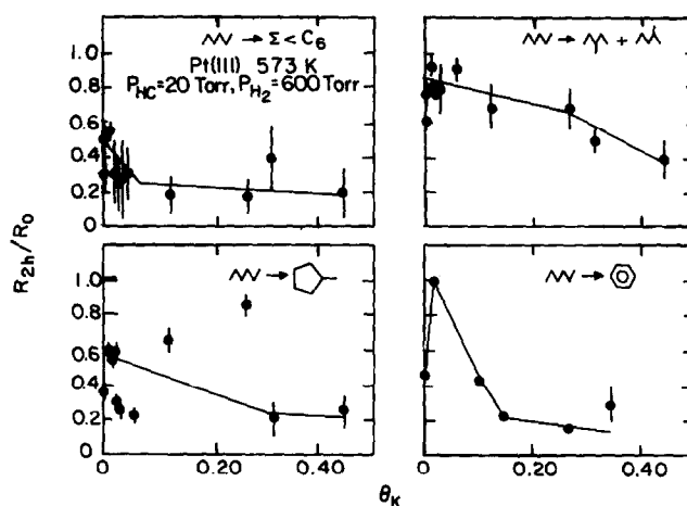
FIG. 4. Stability to self-poisoning, expressed as the ratio of reaction rates after 2 h over initial rates, for hydrogenolysis, isomerization, cyclization, and aromatization of n-hexane over Pt(111) surfaces as a function of potassium coverages.
