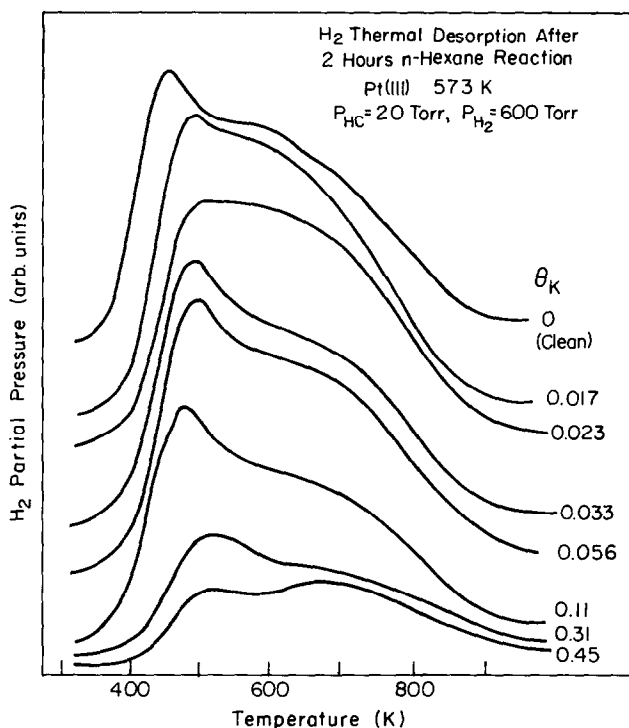
FIG. 9. Hydrogen thermal desorption spectra of the carbonaceous deposits after n-hexane reactions over Pt(111) surfaces with different potassium coverages. Heating rate = 80 K/s.
