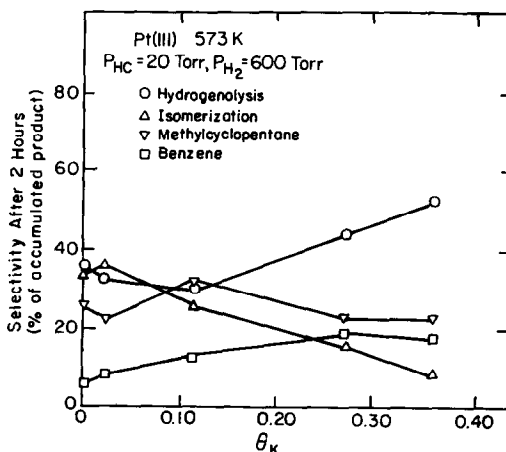
FIG. 3. Selectivity of accumulated products after 2 h of n-hexane reaction over Pt(111) as a function of potassium coverages.
