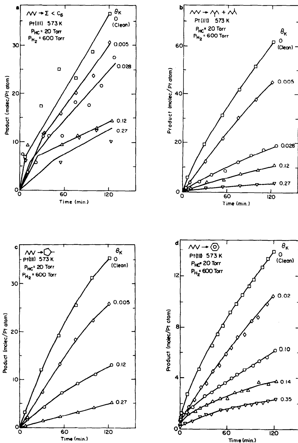
FIG. 1. Product accumulation curves as a function of time for n-hexane reactions over Pt(111) surfaces, dosed with different amounts of potassium: (a) hydrogenolysis, (b) isomerization, (c) methylcyclopentane formation (cyclization), (d) aromatization.
