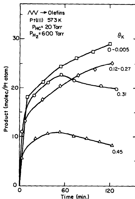
FIG. 5. Product accumulation curves as a function of reaction time for n-hexane dehydrogenation over Pt(111) surfaces covered with different amounts of potassium.
